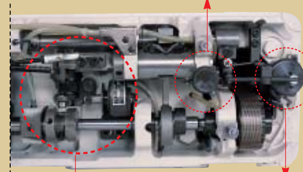
Solenoid-based thread release structure
